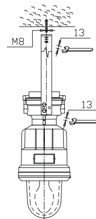
CEILING
